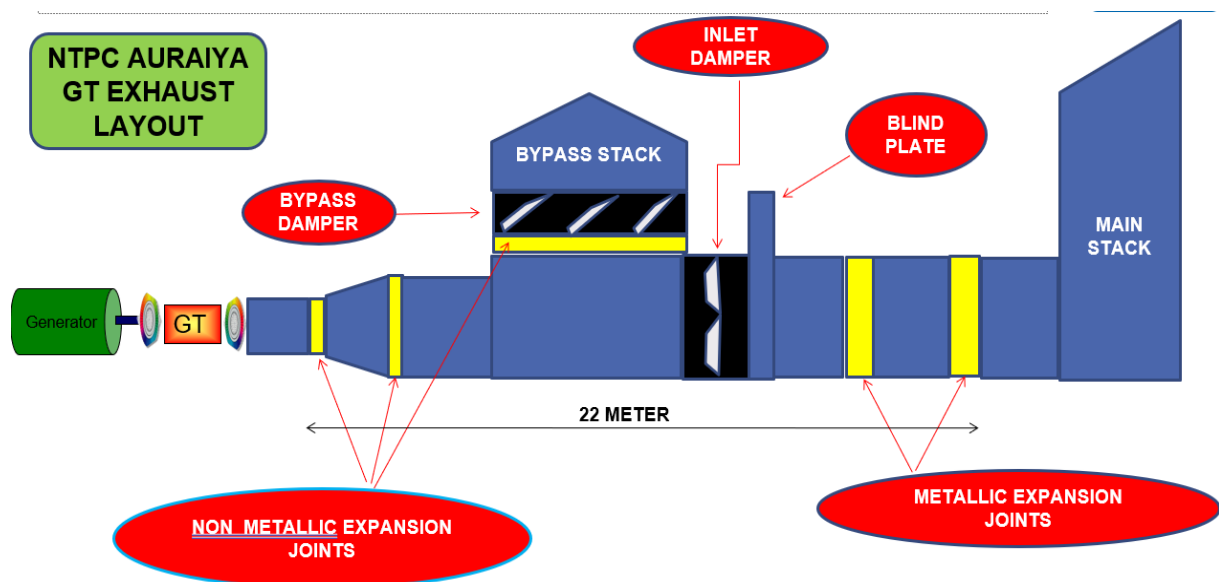
Pictorial representation of existing GT exhaust duct system
